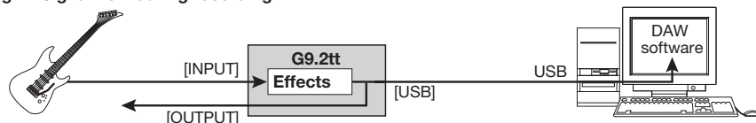
Fig. 2: Signal flow during playback (1)
