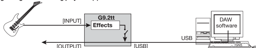
Fig. 3: Signal flow during playback (2)
