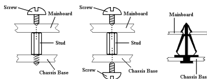
Figure 2-2. The way we fixed the motherboard
