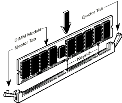
Figure 2-4. Memory module installation
