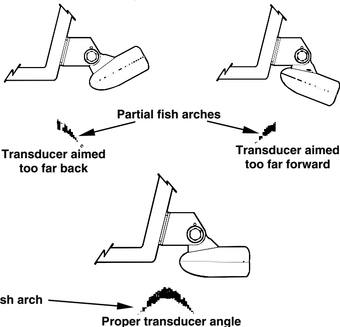
Transducer angles and their effects on fish arches.
