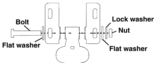
Assemble transducer and bracket.
