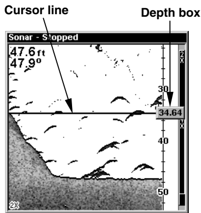
Sonar chart with the depth cursor active. The line indicates the large fish is 34.64 feet deep.
