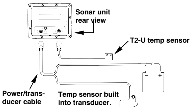
Sonar unit with secondary external temperature sensor.
