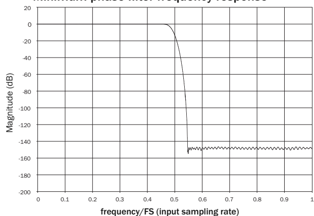
Minimum phase filter frequency response
