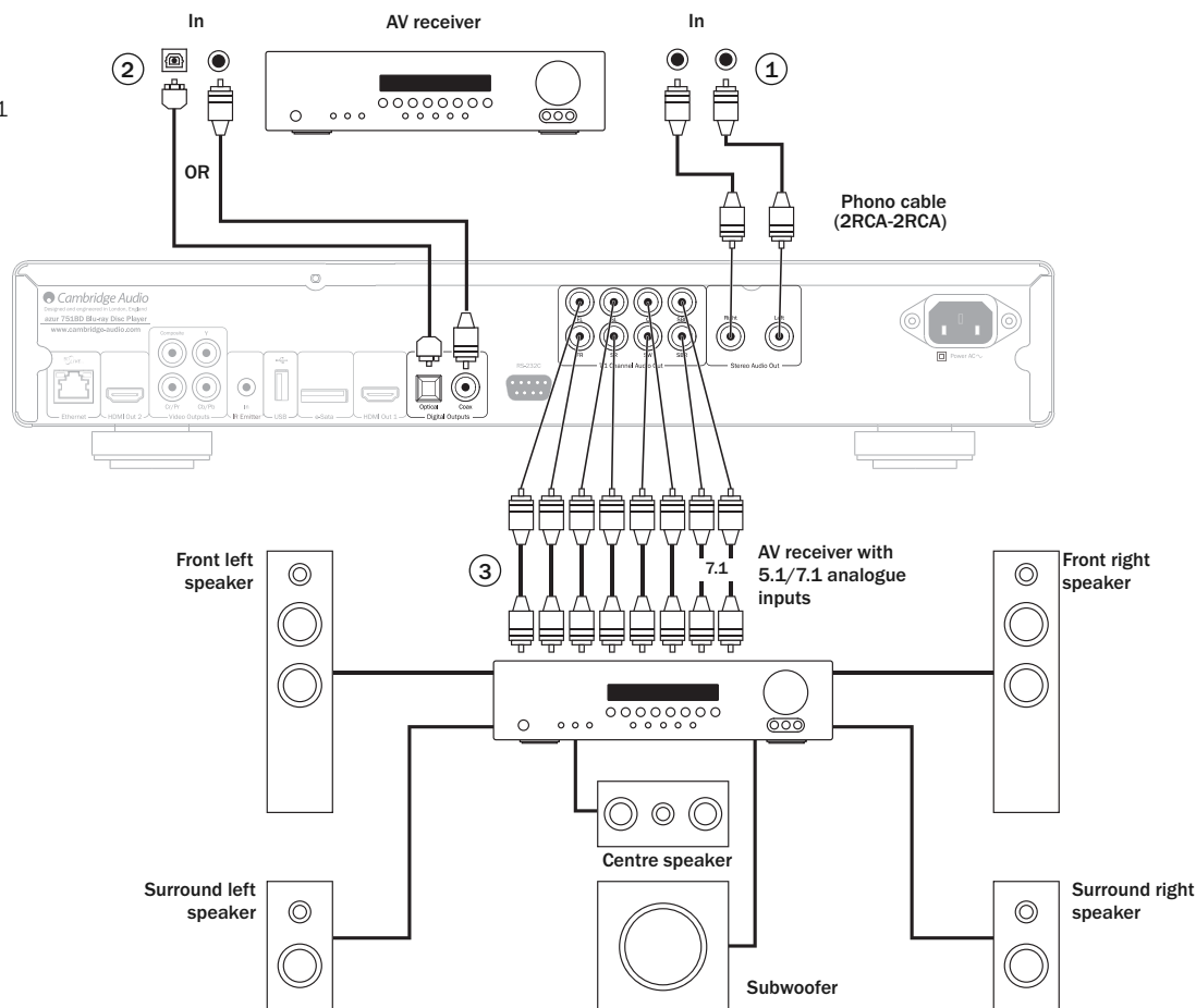
Speaker diagram shown for 5.1 channel setup. For 7.1 add two rear speakers.
