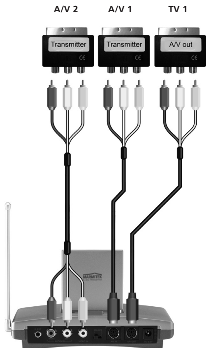
Figure 1 A/V TRANSMITTER
