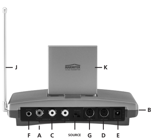
Figure 3 A/V TRANSMITTER
