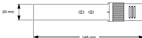
FIGURE 7. DIMENSIONS
