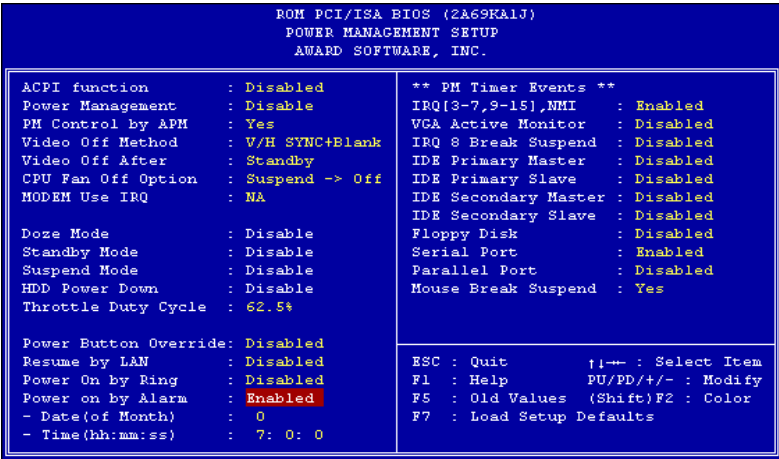
Fig 3-6 Power Management Setup Menu
