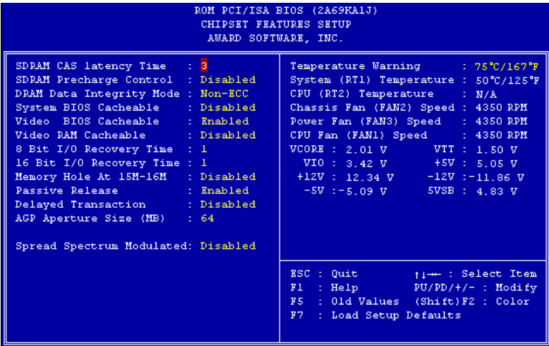
Fig 3-5 Chipset Features Setup
