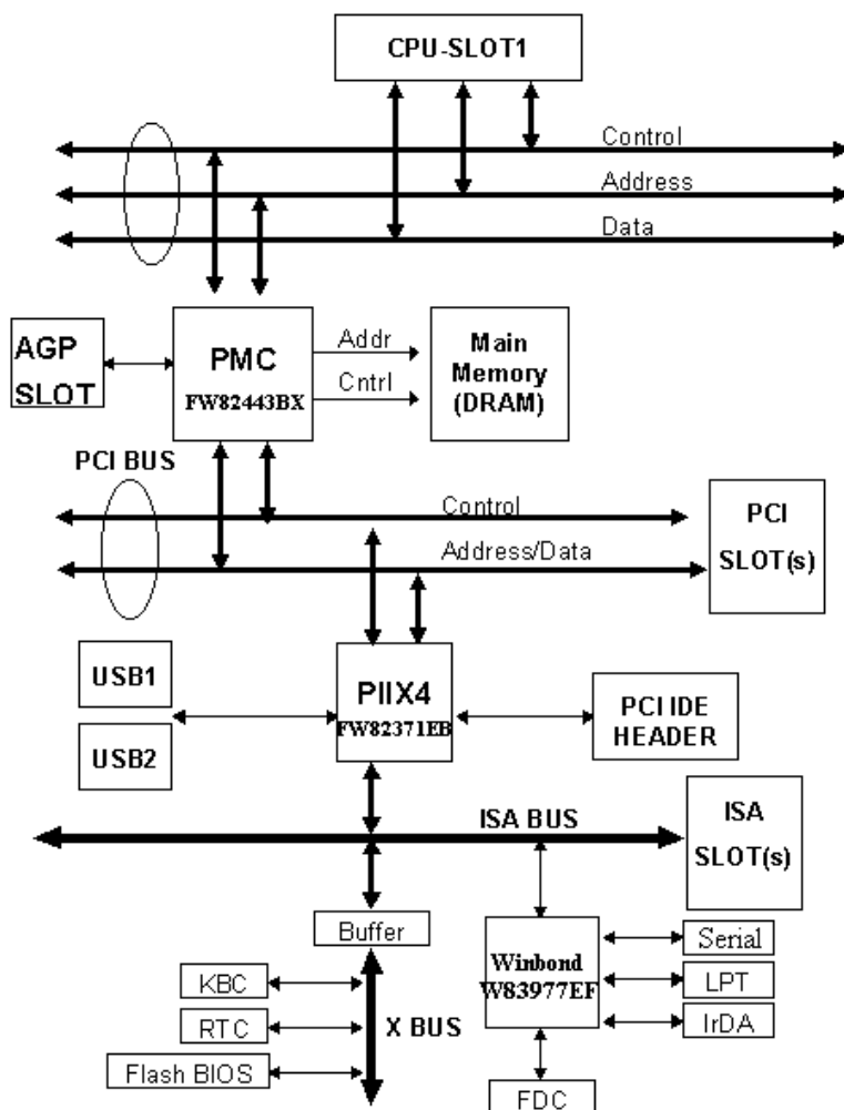
Figure 1-3. System diagram of the 440BX chipset
