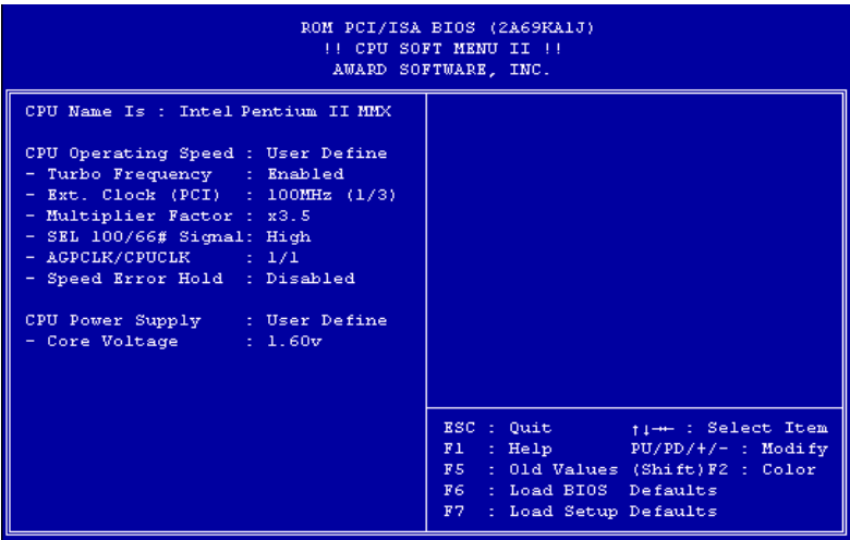
Fig 3-2 CPU SOFT MENU™ II
