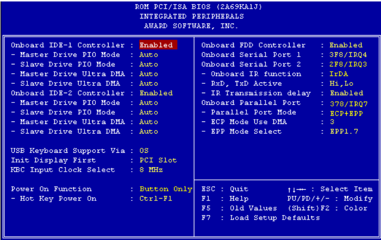
Figure 3-8. Integrated Peripherals Menu
