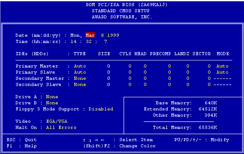
Fig 3-3 Standard CMOS Setup Menu
