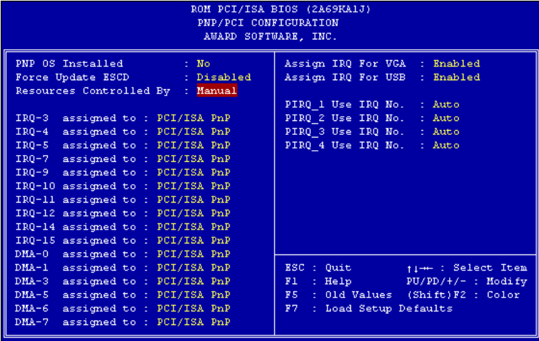
Figure 3-7. PNP/PCI Configuration Menu
