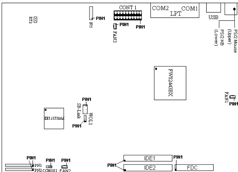
Figure 2-5. All Connectors and Headers for the BX6
