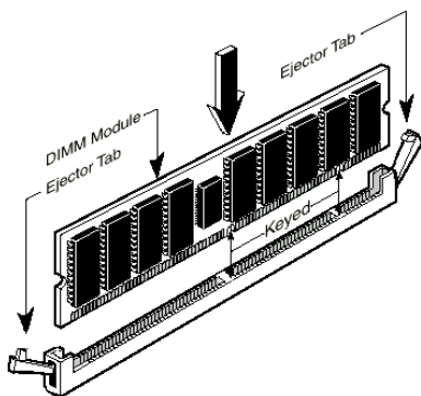
Figure 2-4. Memory module installation
