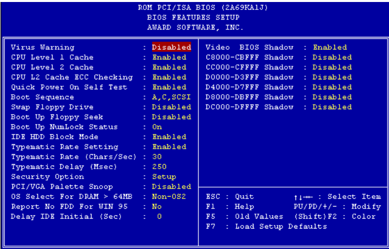
Fig 3-4 BIOS Features Setup
