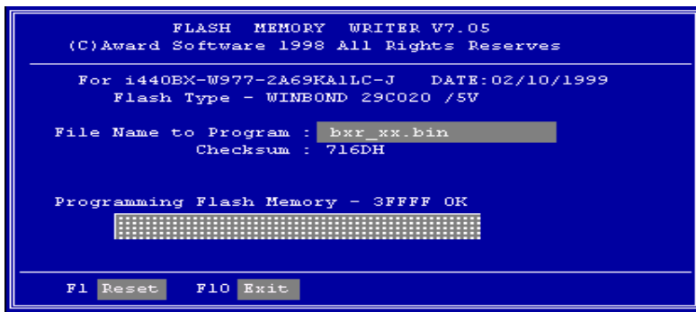
Figure A-2. Ecran Complet d'Award Flash Memory Writer V7.05
