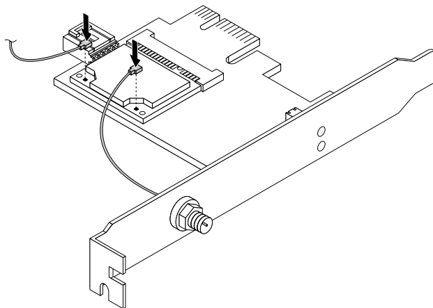
Figure 72. Installation des câbles d'antenne WiFi
