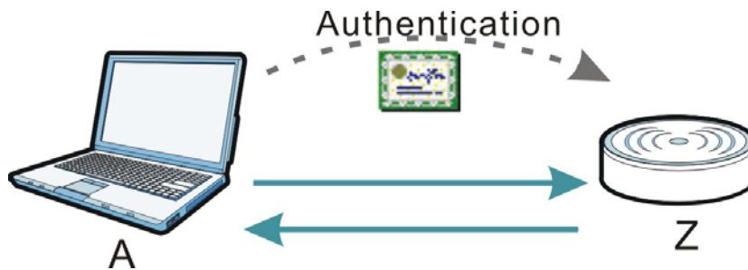
Figure 48 Certificates Example
