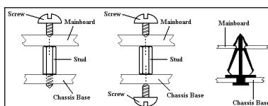
Figure 2-2. Three ways to fix the motherboard onto the chassis
