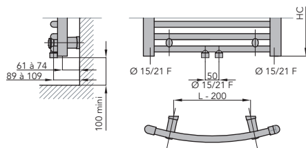
VERSION EAU CHAUDE Raccord Central 50mm
